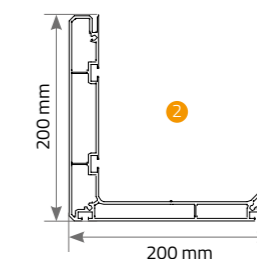
Gutter (Water-drain)
