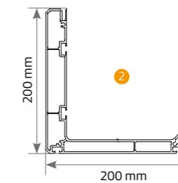
Gutter (Water-drain)
