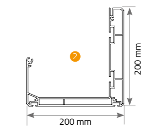
Extruded Frontal Gutter (Water-drain)
